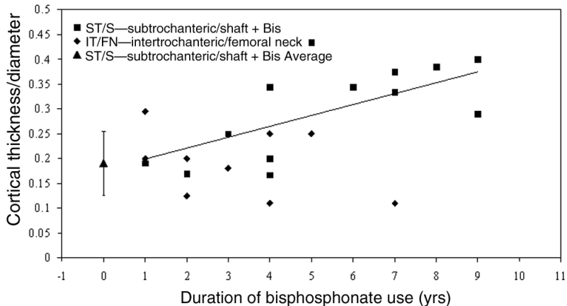
Fig. 2 Cortical thickness to diameter was plotted against duration of bisphosphonate use for all cases on a bisphosphonate. The ratio of the cortical thickness to diameter increased as the duration of bisphosphonate use increased. This relationship was not seen for cases not on a bisphosphonate or for controls on a bisphosphonate.
